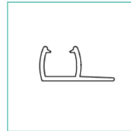
6mm Vertical Flap with 15mm Leg PGFVL15-6
